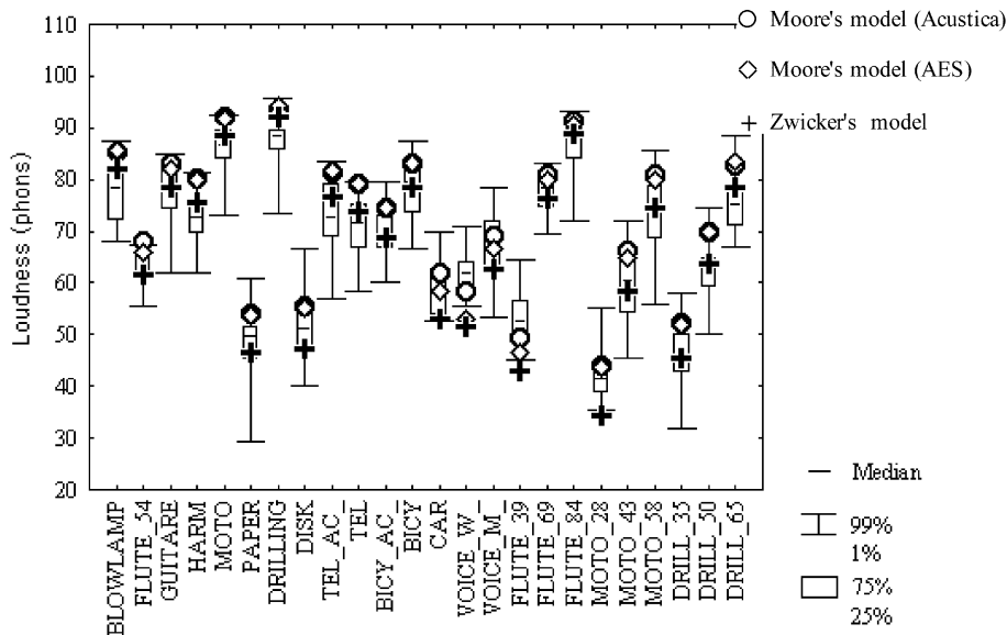
Fig. 3 : Adjusted loudness of each of the twenty-four environmental sounds. The Box Whiskers places a box around the median (horizontal line) which represents the 75th percentile and whisker outside of the box represent the 99th percentile. The symbols are the prediction of the three models, as indicated next to the figure.
