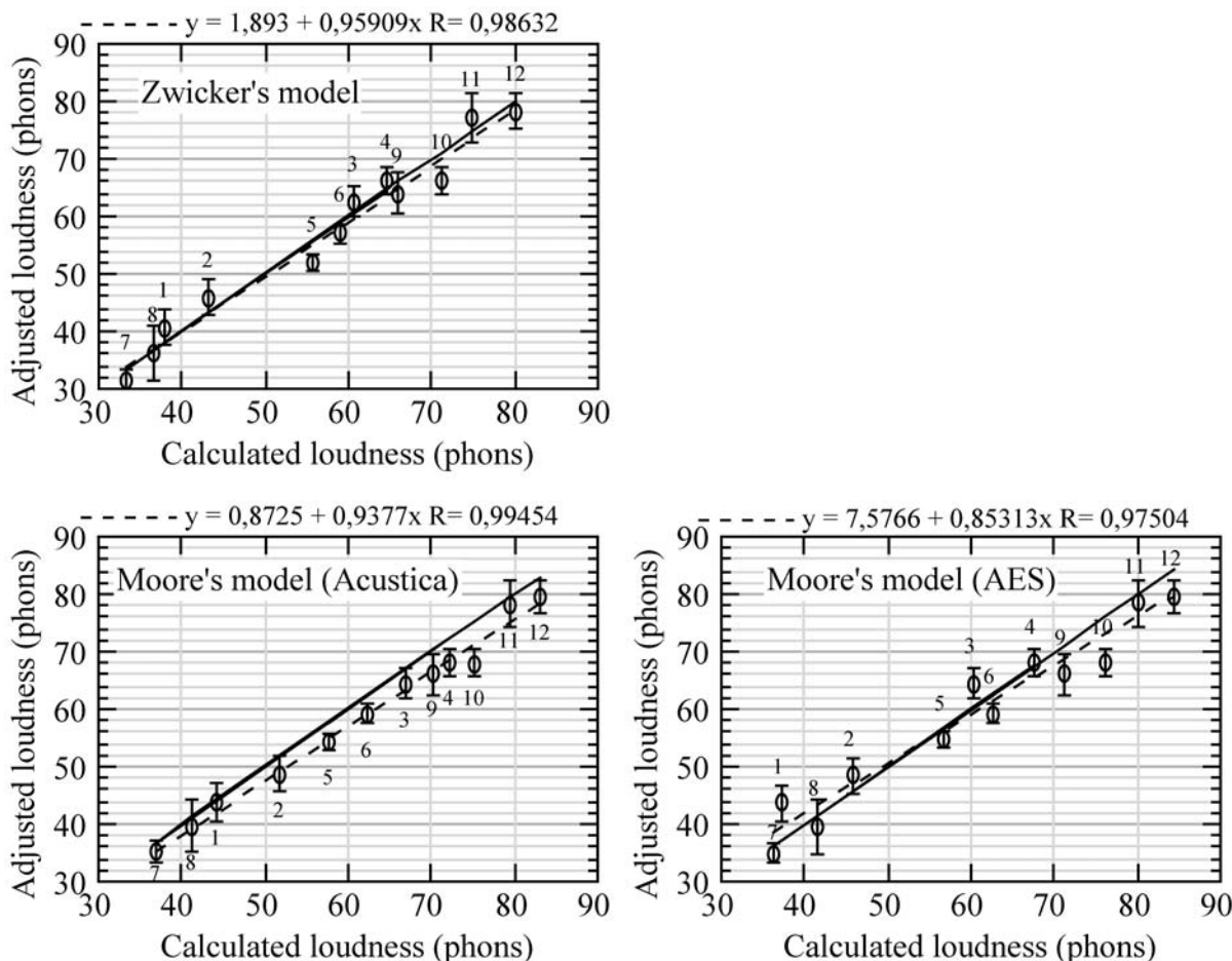
Fig. 1 : Adjusted loudness as a function of the calculated loudness for the synthesized noises: The top graph shows the comparison with Zwicker's model. The bottom graphs show the comparison with Moore's models. open circles - adjusted loudness; solid line - predictions of the model; dashed line - fitting with the data. The number next to the symbols are the sound numbers.
