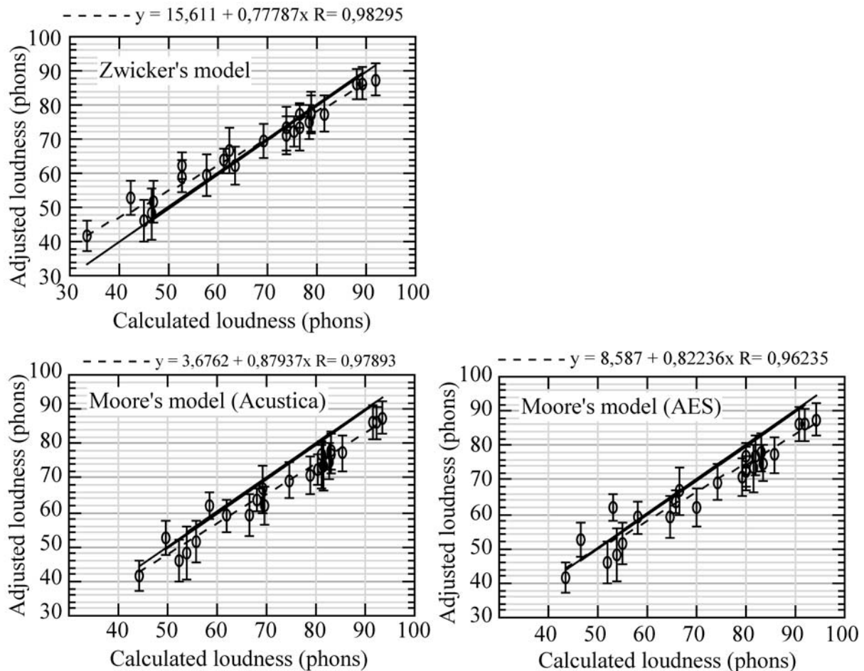
Fig. 2 : Adjusted loudness as a function of the calculated loudness for the environmental sounds: the symbols are the same as in Fig.1.
