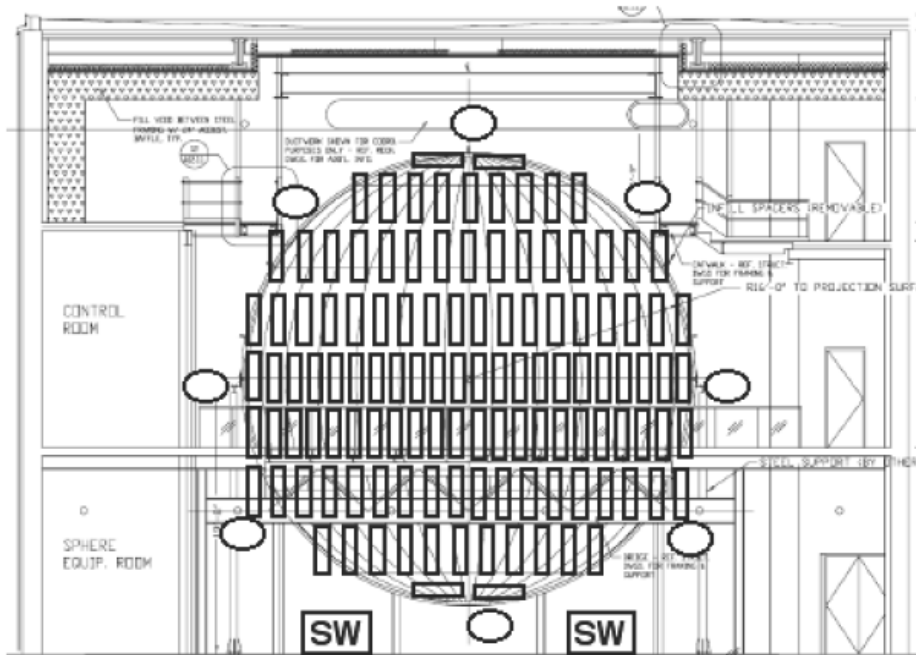
Fig. 7. Allosphere speaker placement design, initial results after first iterations taking into account VBAP requirements
