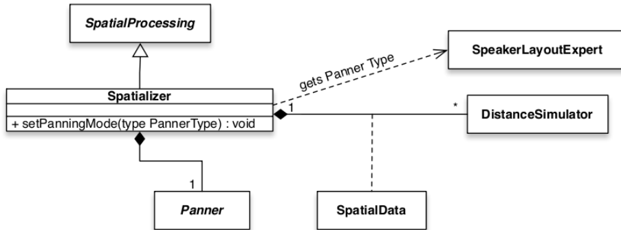
Fig. 8. Spatializer Class Diagram
