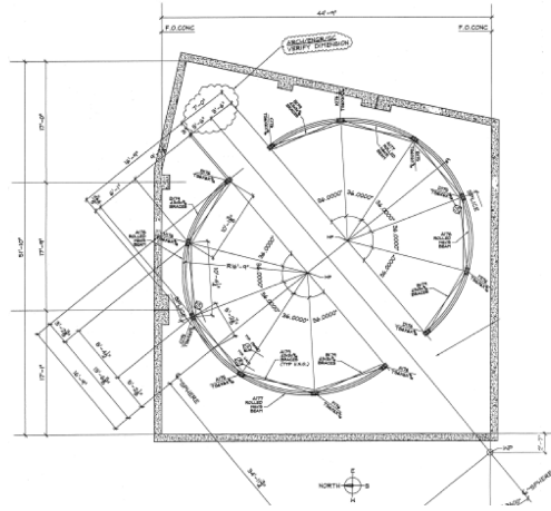
Fig. 4. Horizontal section of the Allosphere
